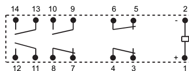
Wiring Diagram (Bottom view)
